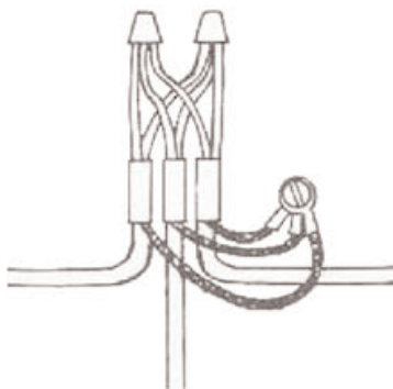
Tee Splice
