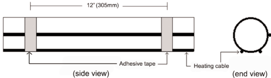
Straight run
